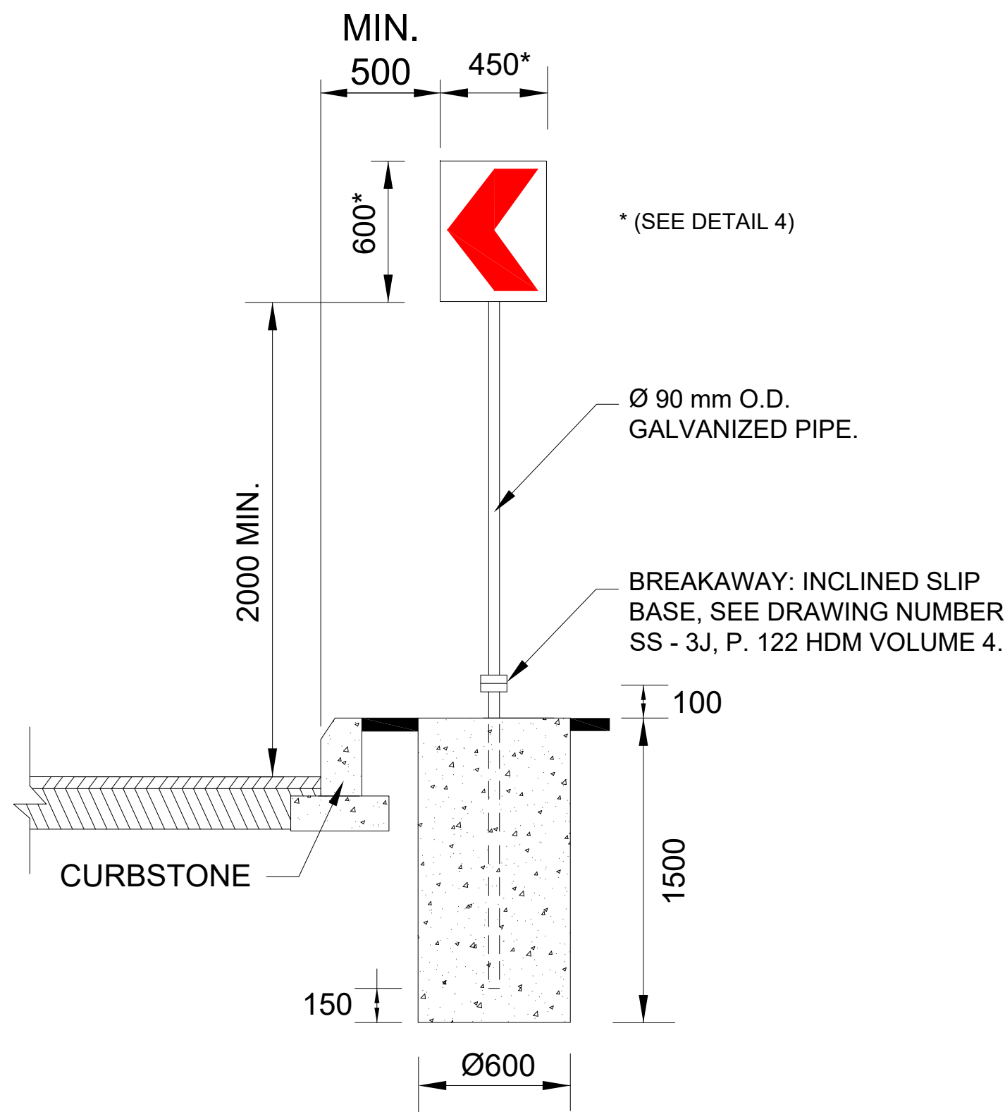
3 TYPICAL INSTALLATION DETAILS IN URBAN AREA ROADWAYS
