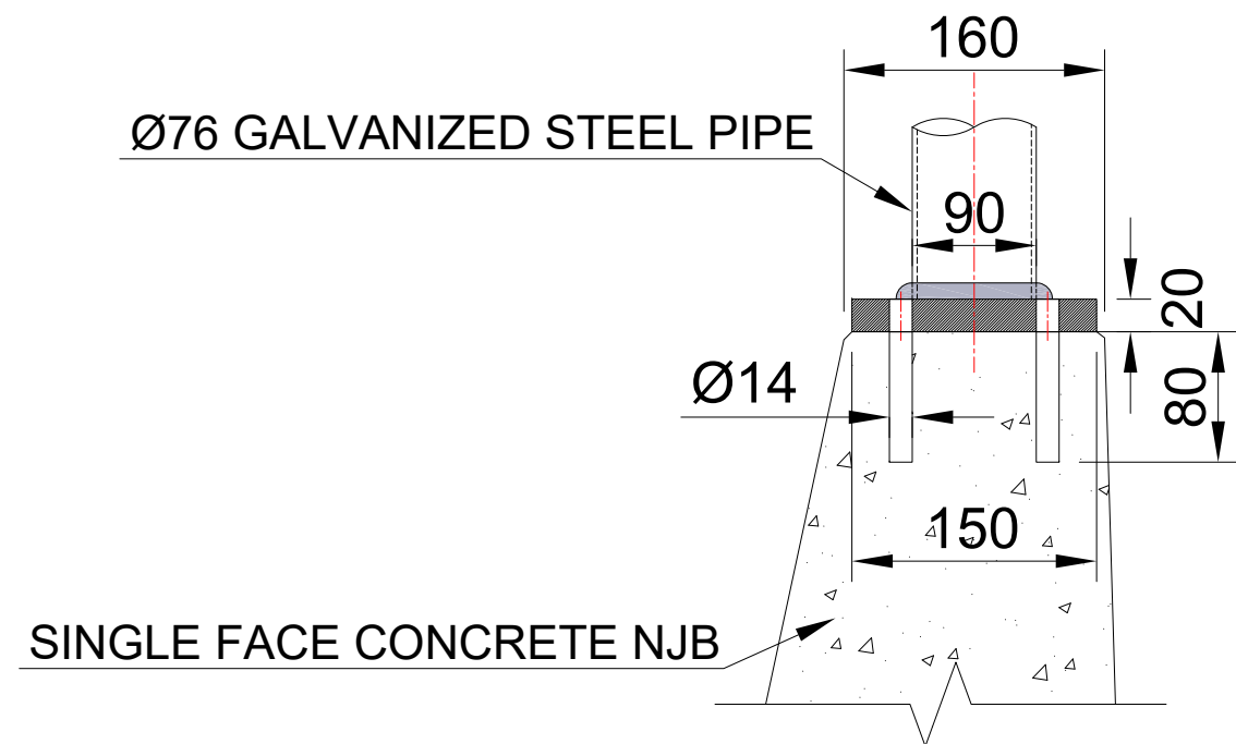
ELEVATION SECTION A-A SIGN POST FIXATION DETAILS ON CONCRETE NEW JERSEY BARRIER
