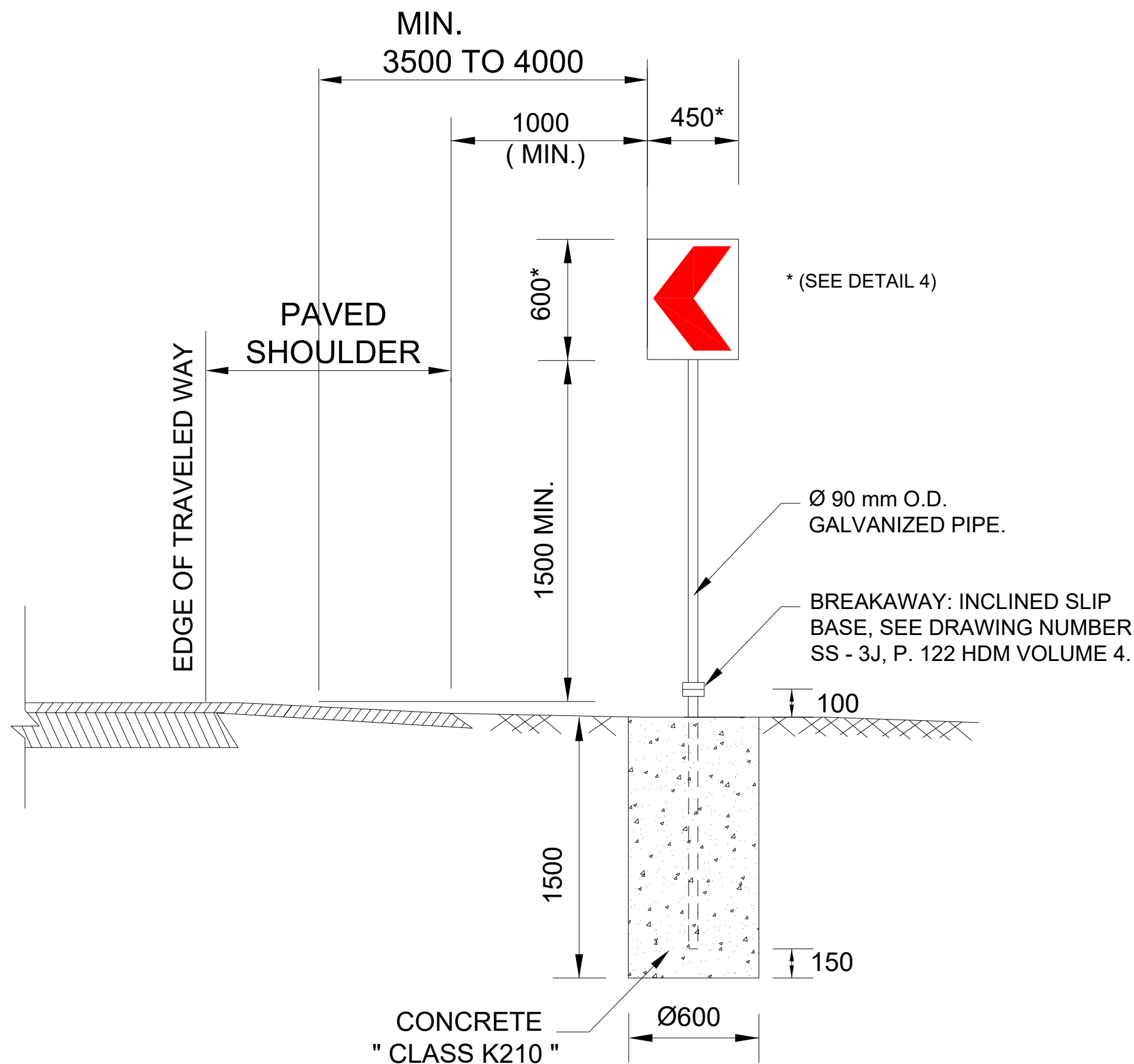
1 TYPICAL INSTALLATION DETAILS IN RURAL AREA ROADWAYS
