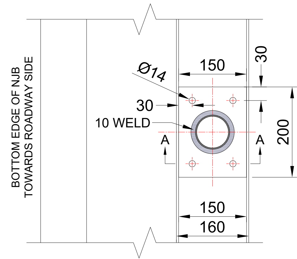
PLAN SECTION B-B SIGN POST FIXATION DETAILS ON CONCRETE NEW JERSEY BARRIER
